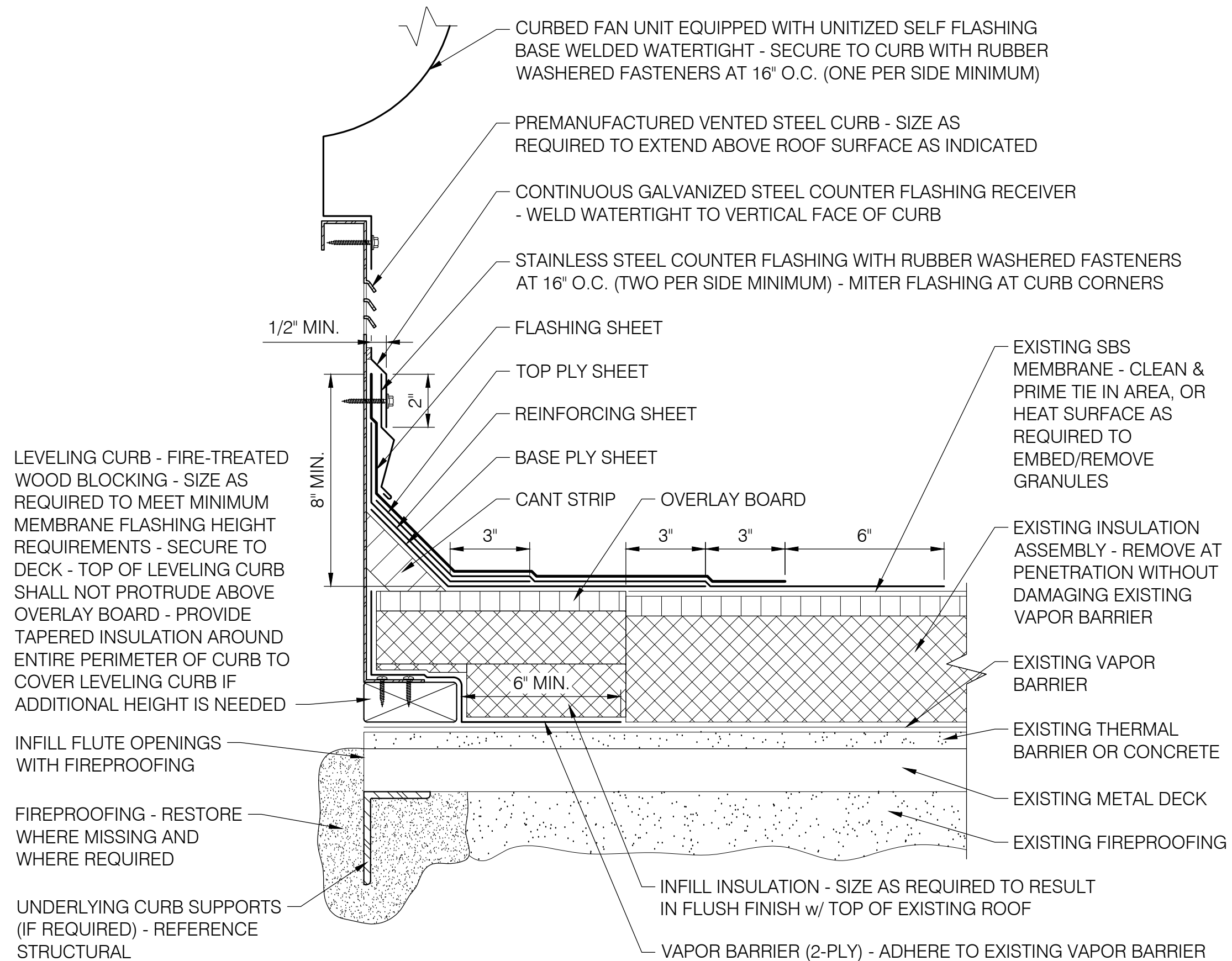
0705 SBS CURB - VENTED FAN UNIT SCALE: 3" = 1'-0"
