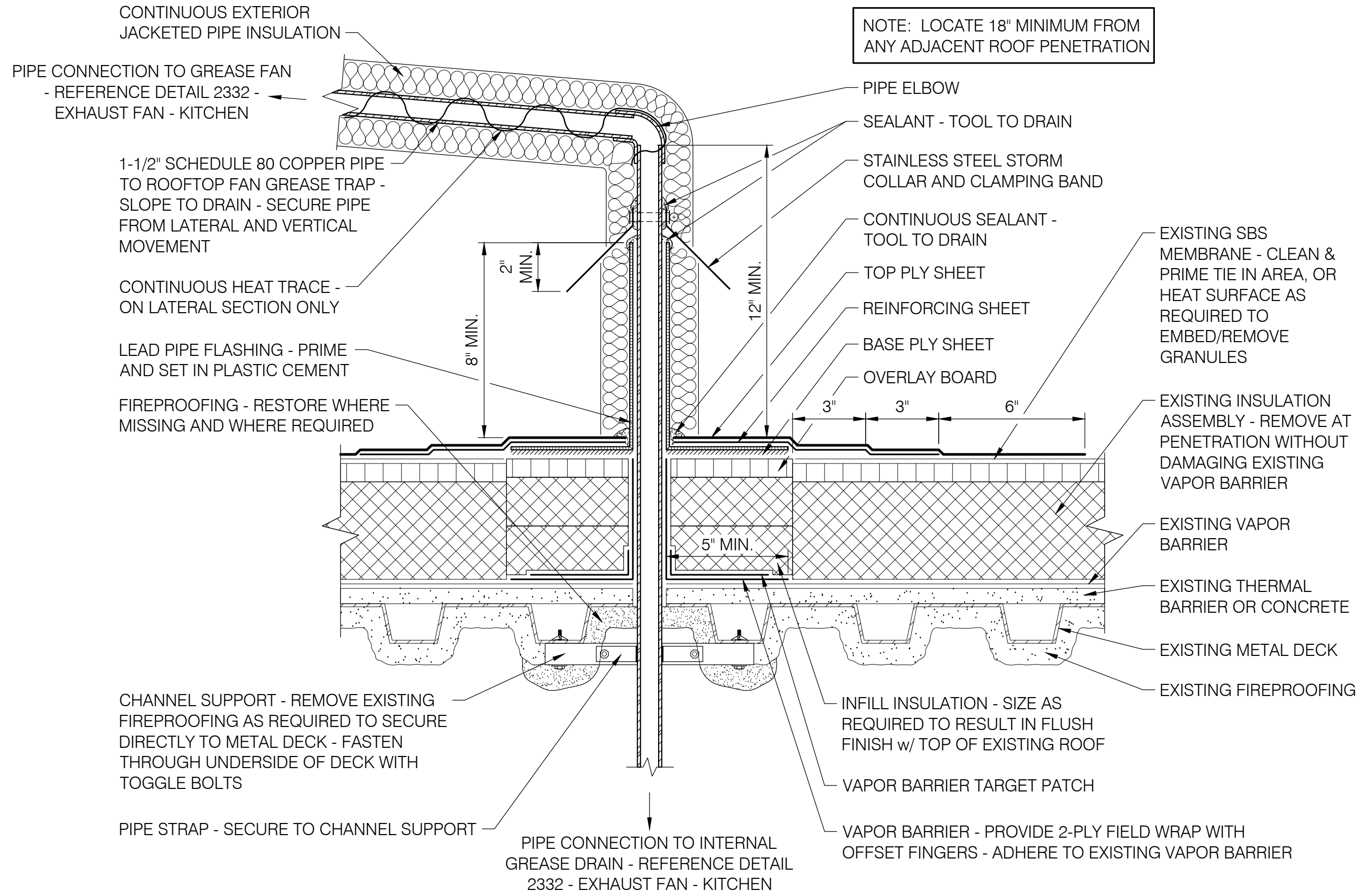
0714 SBS FLASHING - GREASE DRAIN LINE SCALE: 3" = 1'-0"
