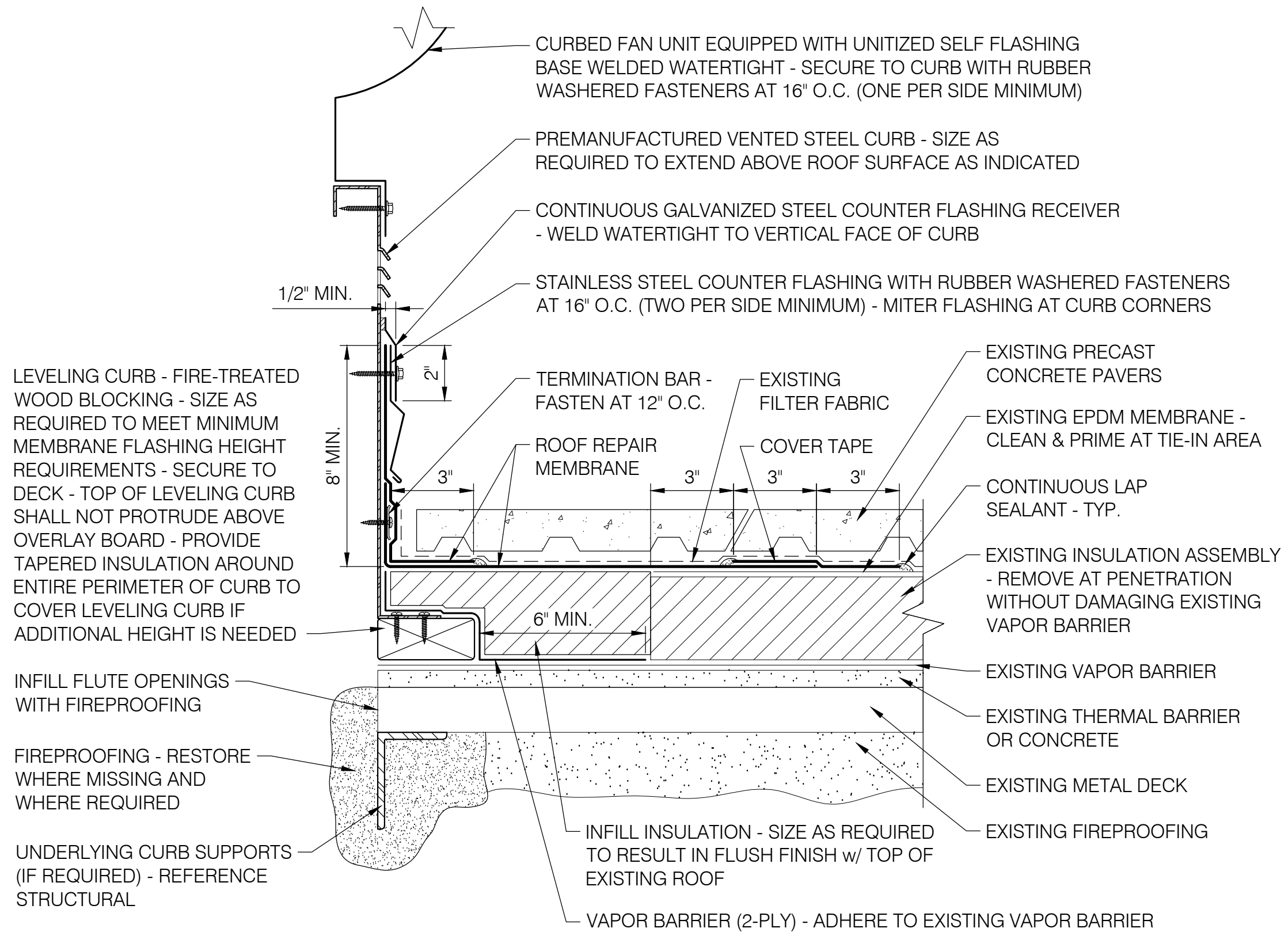
0725 EPDM CURB - VENTED FAN UNIT SCALE: 3" = 1'-0"
