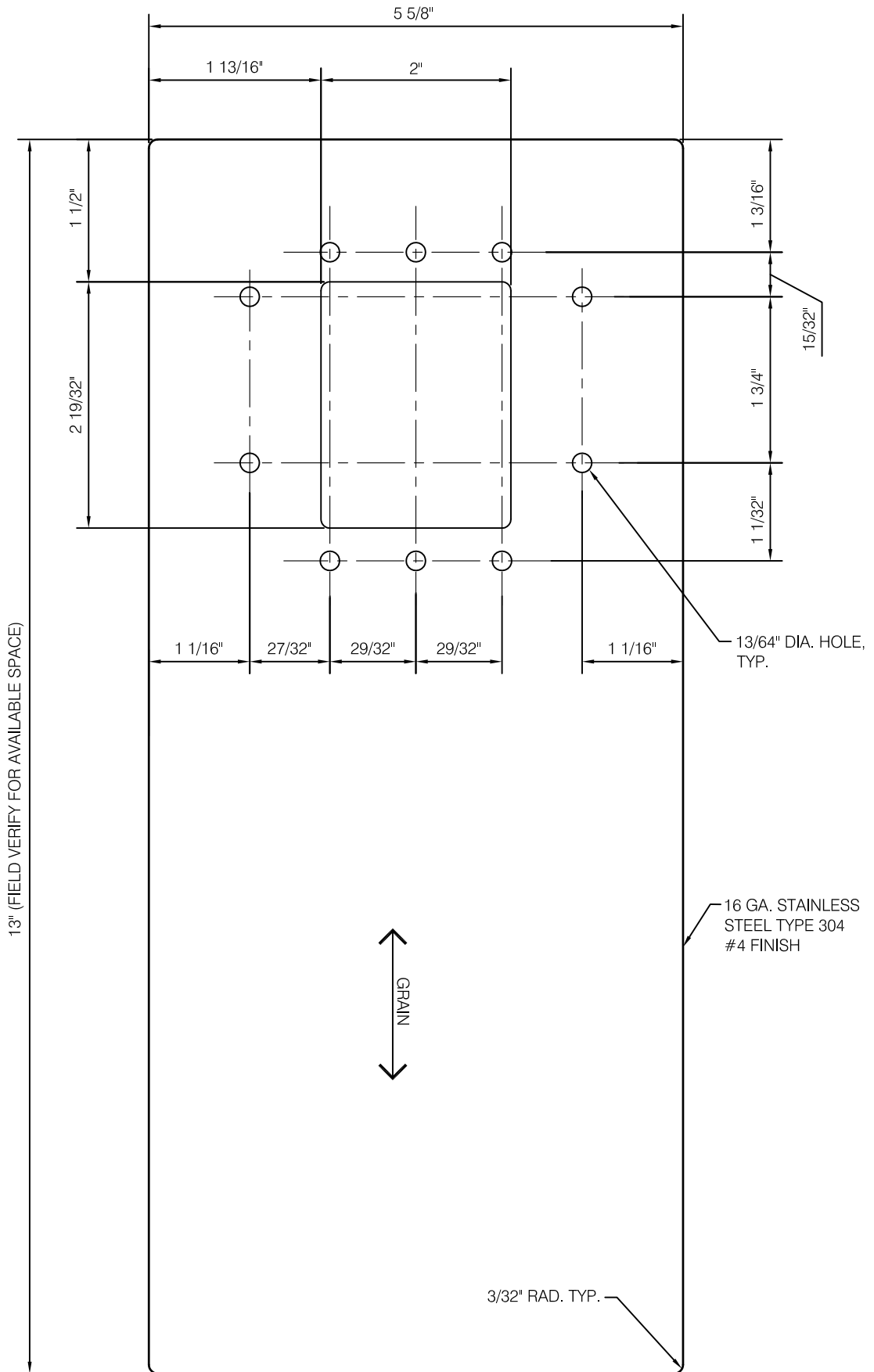
0504 CARD SWIPE BACKPLATE SCALE: NTS
