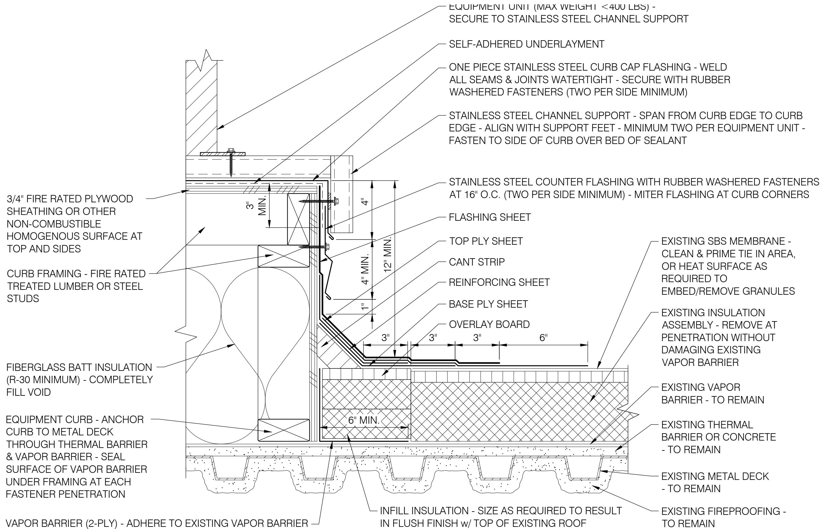
0702 SBS CURB - EQUIPMENT < 400 LBS. SCALE: 3" = 1'-0"
