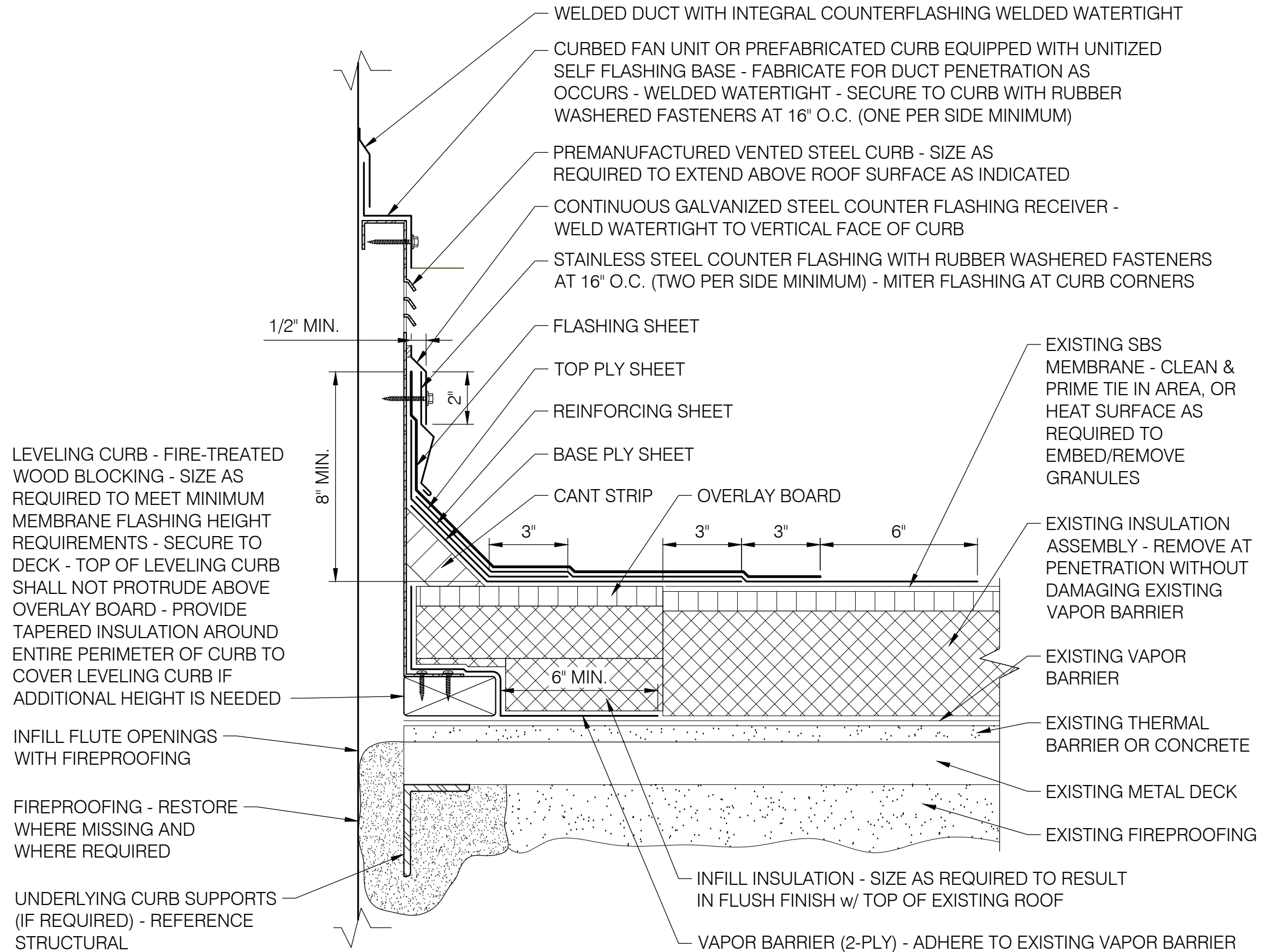
0705 SBS CURB - VENTED FAN UNIT SCALE: 3" = 1'-0"
