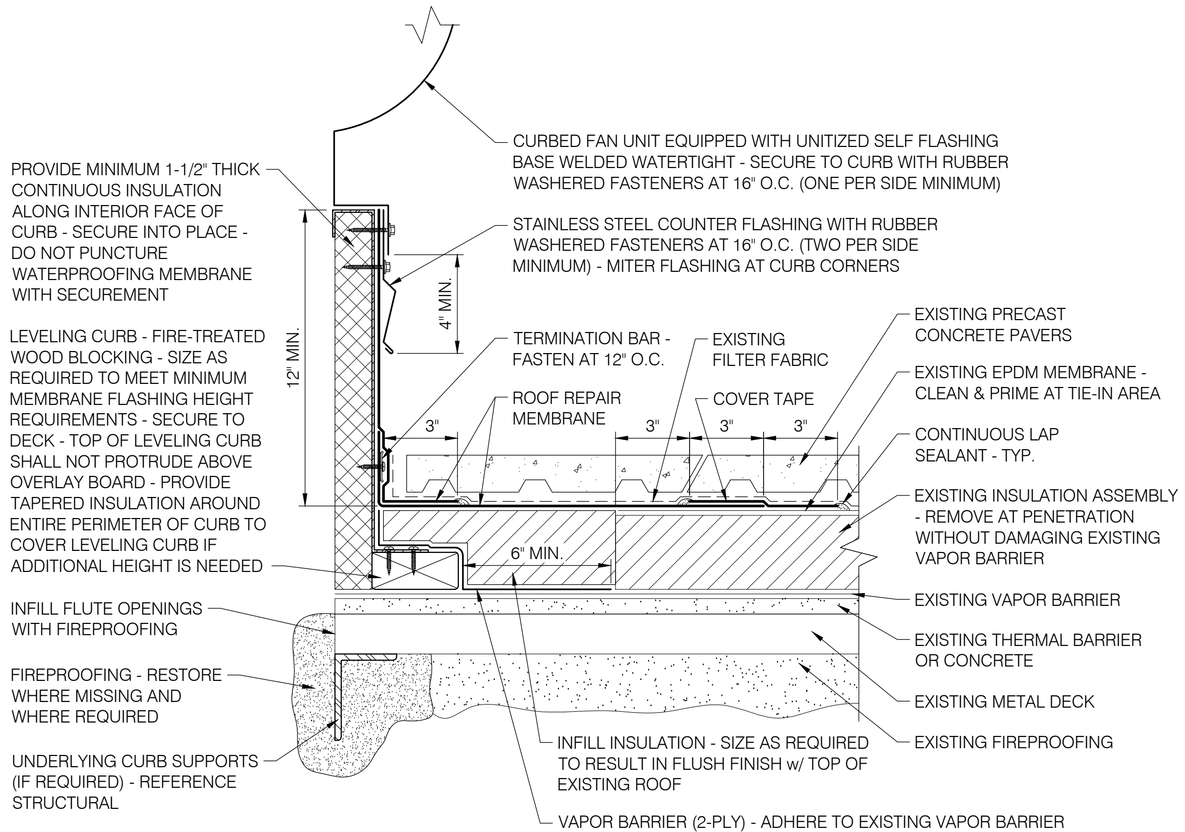
0724 EPDM CURB - UNVENTED FAN UNIT SCALE: 3" = 1'-0"
