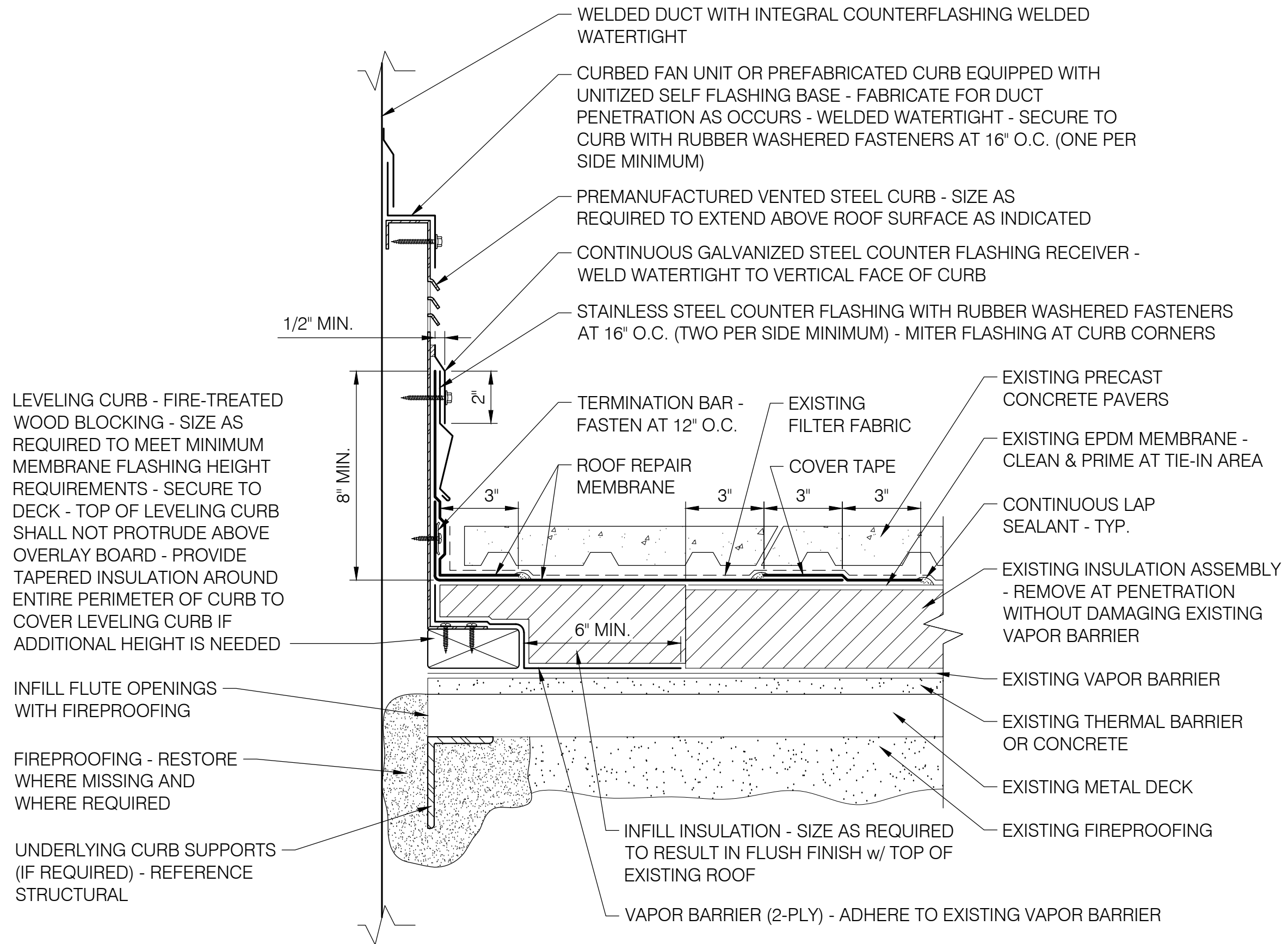
0725 EPDM CURB - VENTED FAN UNIT SCALE: 3" = 1'-0"
