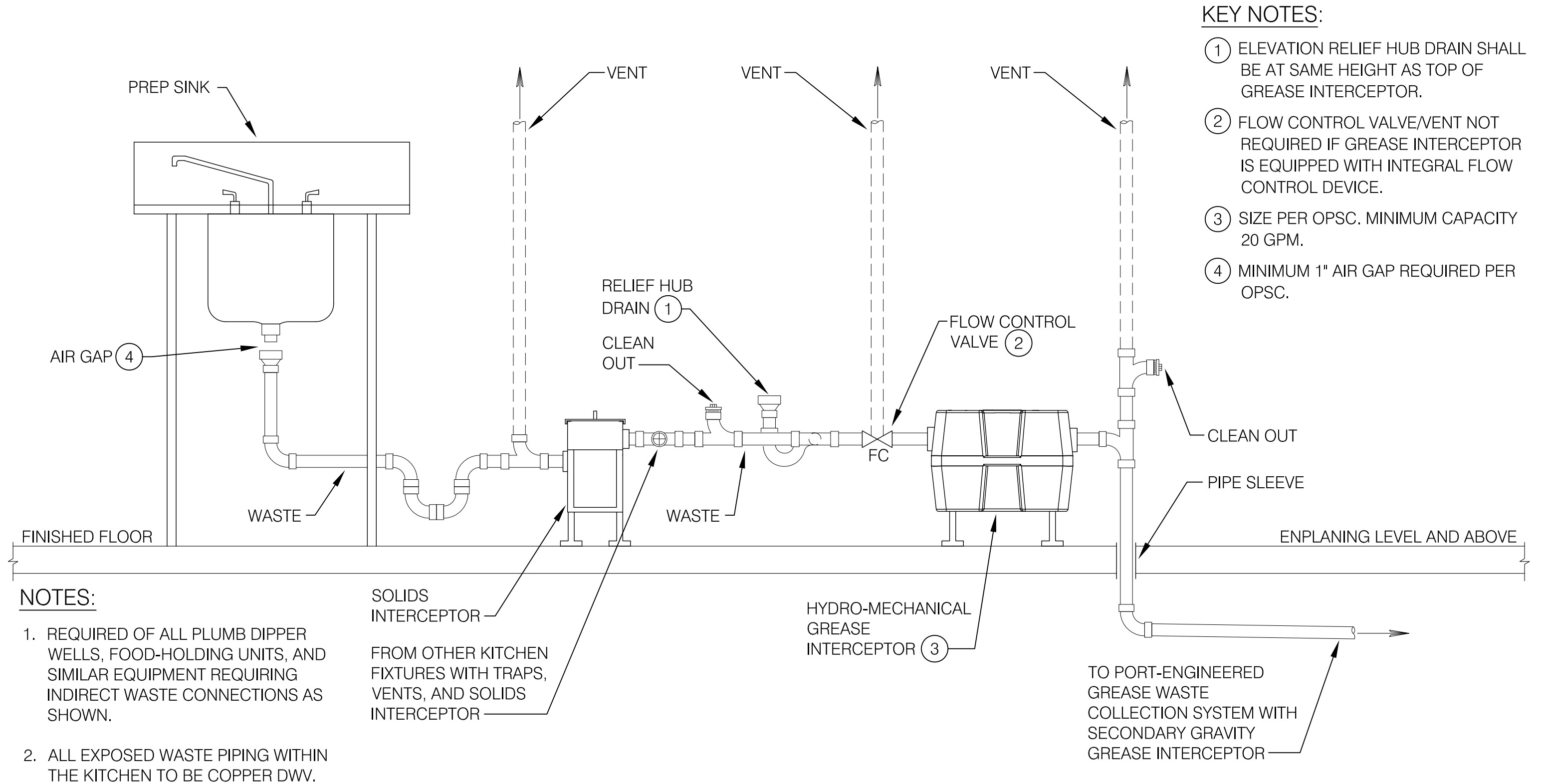
2211 SINK - FOOD PREP OR INDIRECTLY DRAINED EQUIPMENT SCALE: NTS
