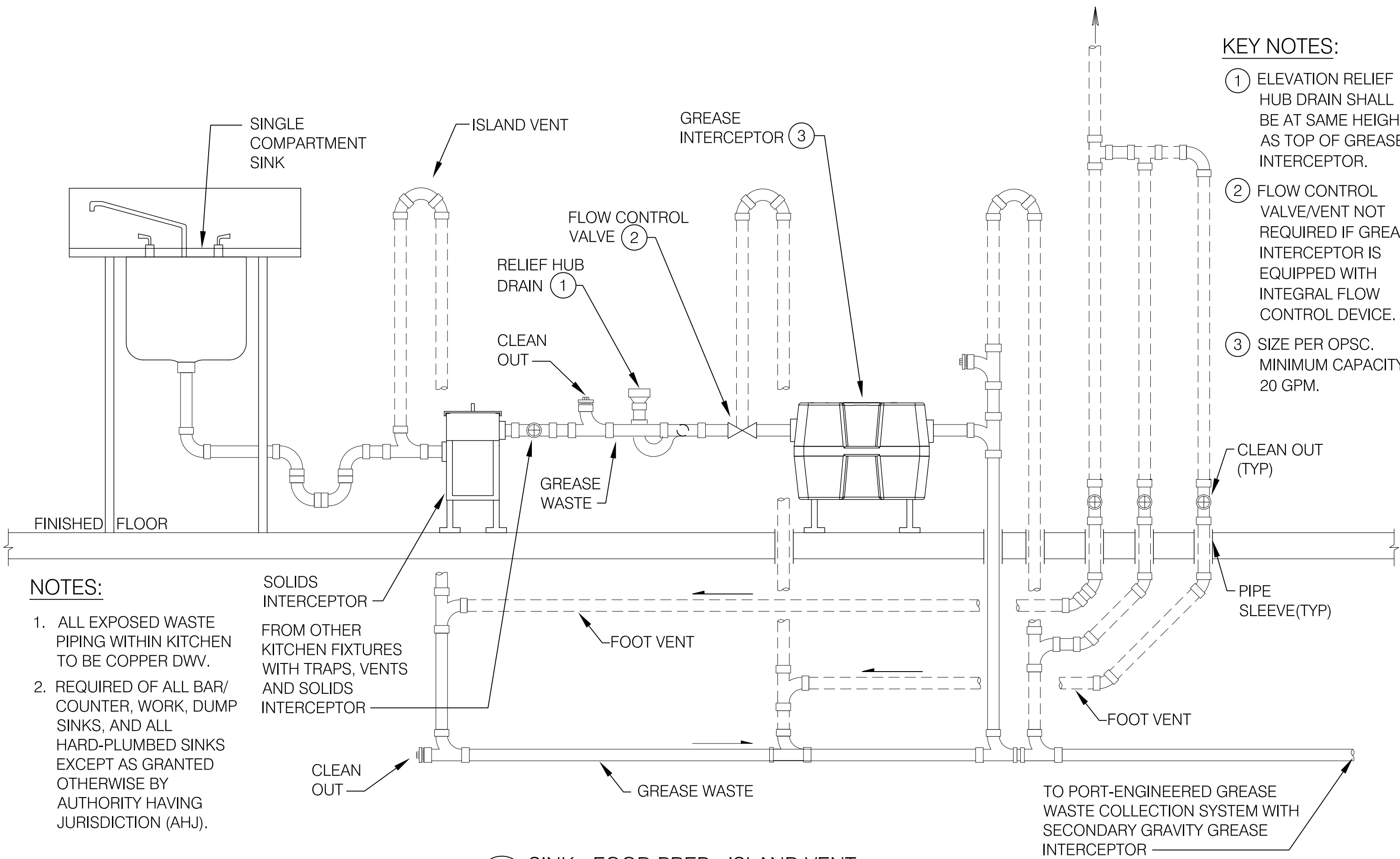
2216 SINK - FOOD PREP - ISLAND VENT SCALE: NTS
