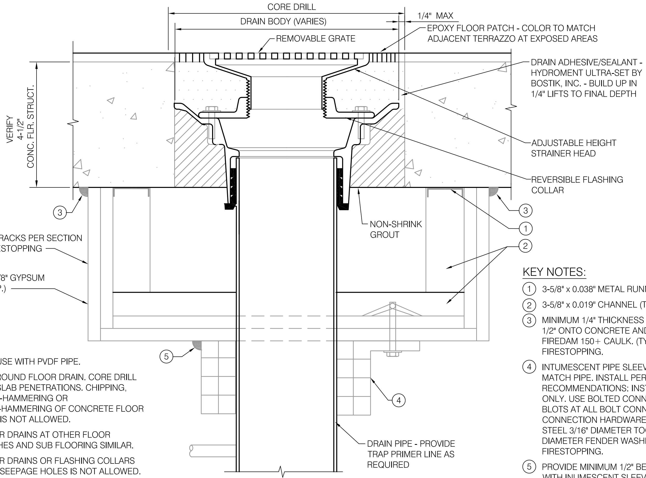
2224 FLOOR DRAIN - CONCRETE FLOOR - PVDF PIPE SCALE: NTS
