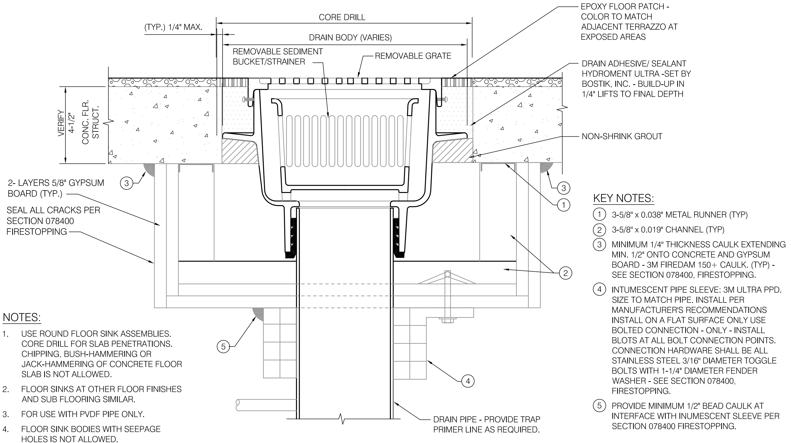
2234 FLOOR SINK - CONCRETE FLOOR - PVDF PIPE SCALE: NTS
