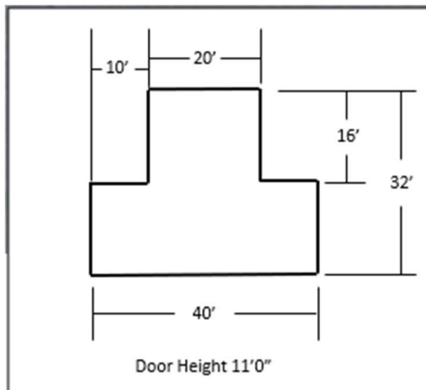
Small Hangar- 960 sq ft
