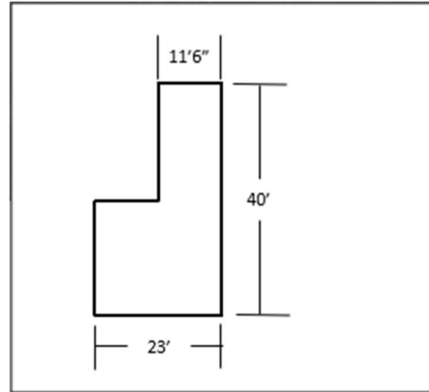
Half-Hangar C19/C36
